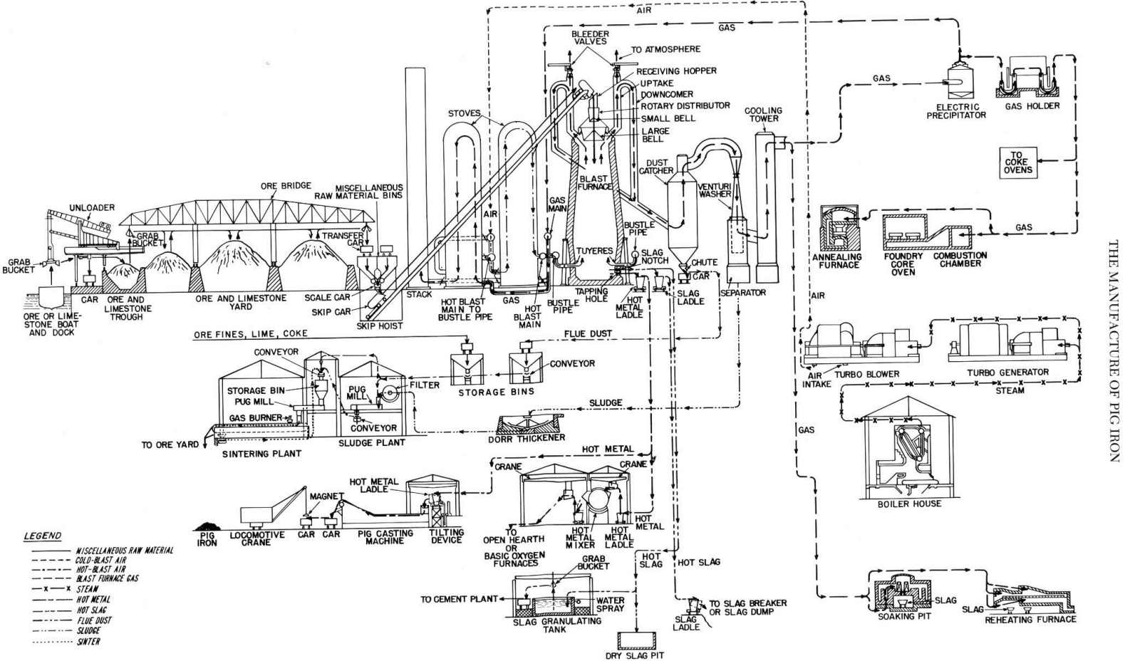
FIG. 15—2. Flow diagram depicting the principal units and auxiliaries in a modern blast-furnace plant, and showing the steps in the manufacture of pig iron from receipt of raw materials to disposal of pig iron and slag, as well as the methods for utilizing the furnace gases.
