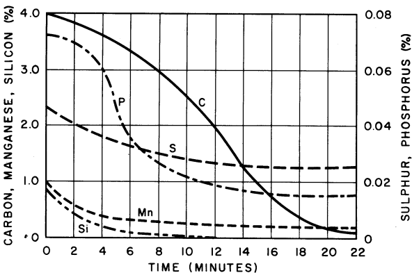
FIG. 16—18. Schematic representation of progress of refining in a top-blown basic-lined vessel.
